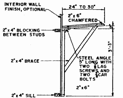
SPACE RACKS 24" TO 30" APART SADDLE RACK
