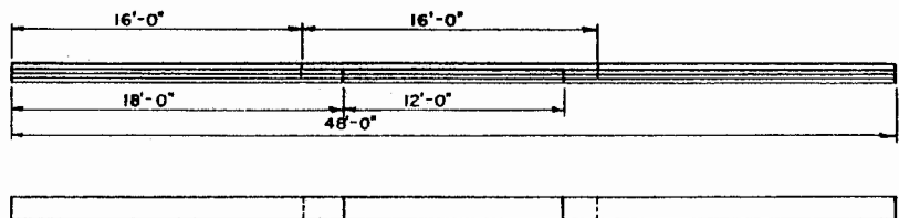
GIRDER LAMINATION DETAIL
