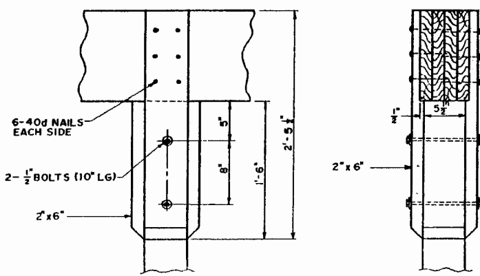
POST & GIRDER DETAIL
