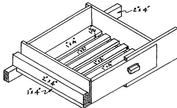
ISOMETRIC - SHOWING CONSTRUCTION OF DRAWER
