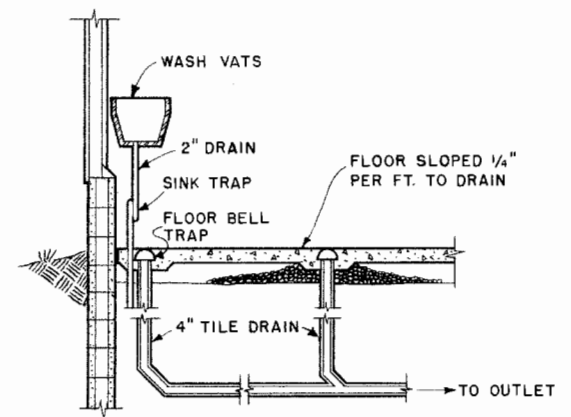
WASH VATS AND DRAIN SECTION
