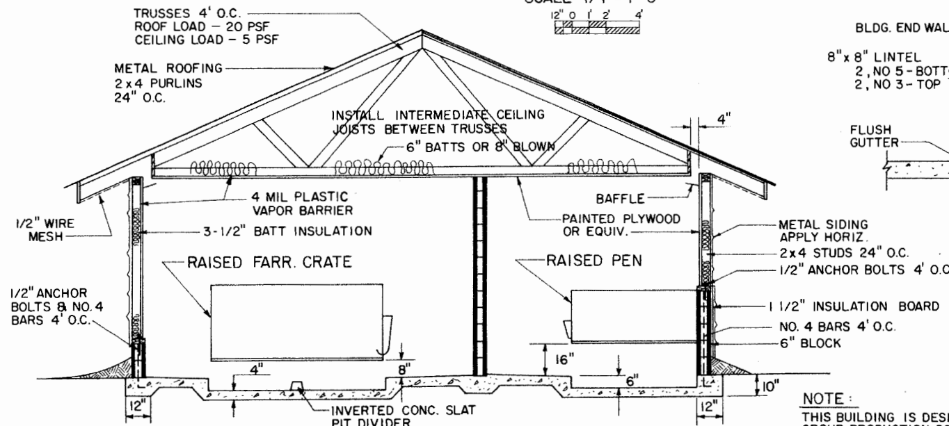
TYPICAL SECTION SCALE: 3/8" = 1'-0"
