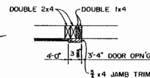
④ SECTION AT DOOR
