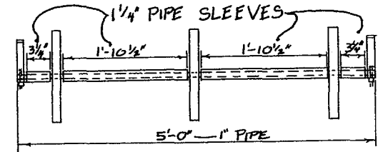
WHEEL ROD
