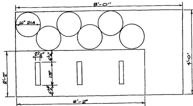
PLYWOOD LAYOUT
