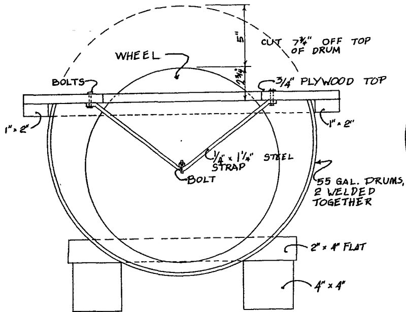
CROSS SECTION
