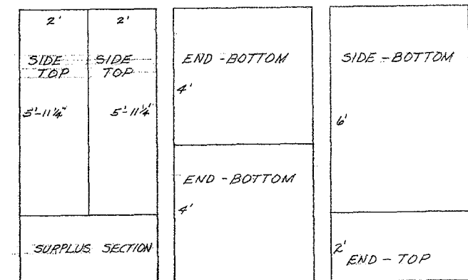
4' x 8' PLYWOOD 1 SHEET REQD. 4' x 8' PLYWOOD 1 SHEET REQD. 4' x 8' PLYWOOD 2 SHEETS REQD. PLYWOOD LAYOUT
