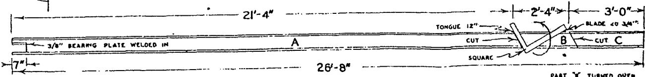
H-BEAM CUTS
