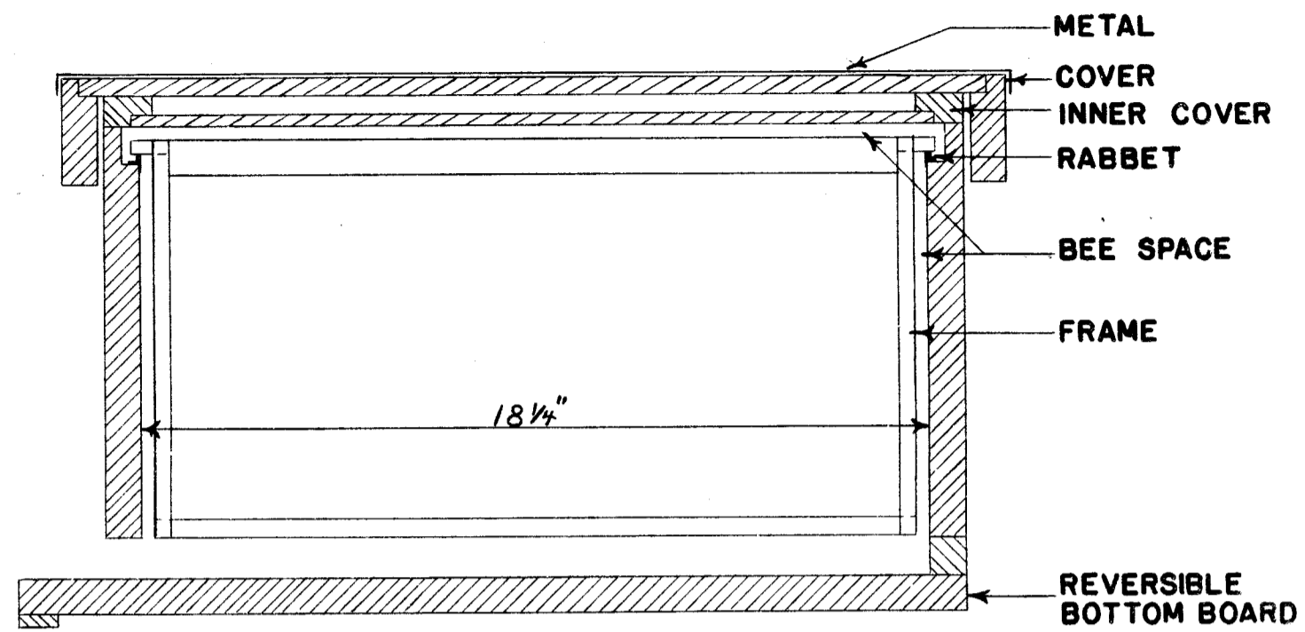
CROSS SECTION OF HIVE BODY AND FRAME:
