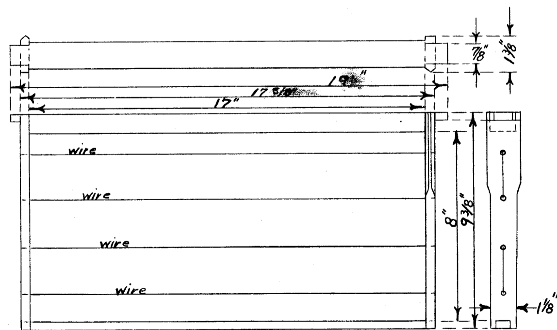
TOP, SIDE, AND END ELEVATION OF FRAME:
