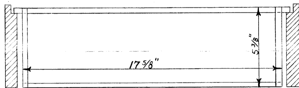
CROSS SECTION OF SHALLOW SUPER:
