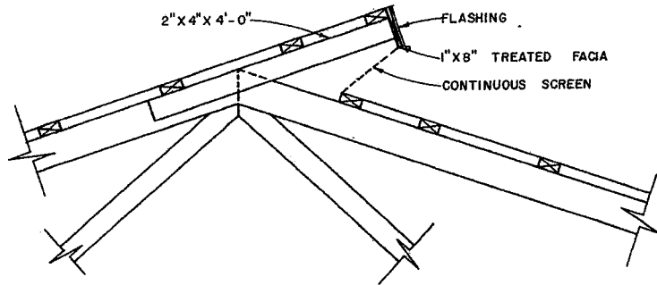
RIDGE - VENT DETAIL
