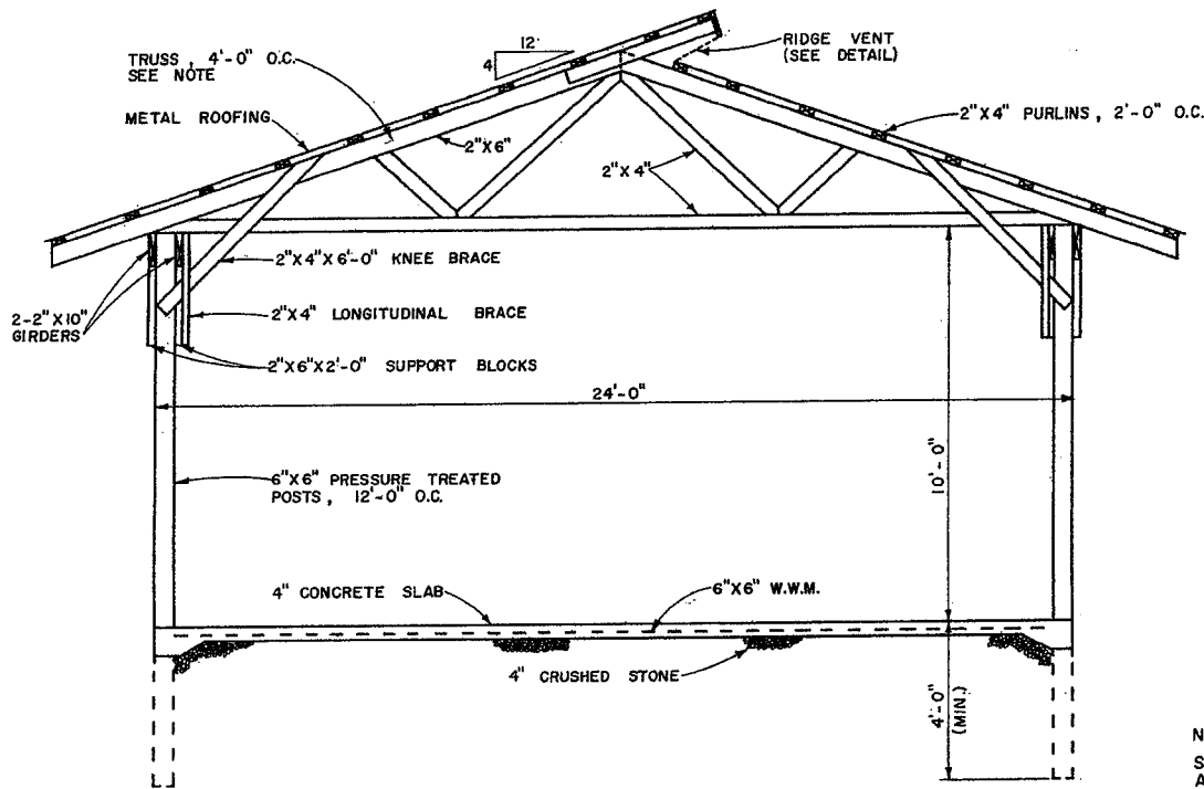
CROSS SECTION
