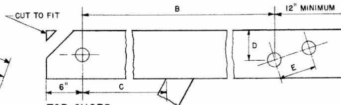
TOP CHORD
