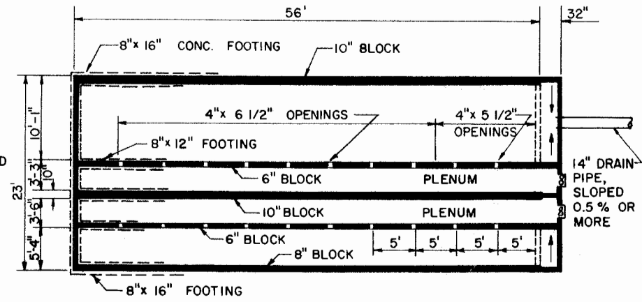
FOUNDATION PLAN SCALE: 1/8" = 1'-0"
