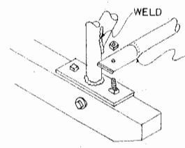
SKID CONNECTION DETAIL (STRUTS ARE REMOVED AFTER MOVING)
