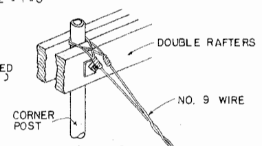
X-BRACING DETAIL
