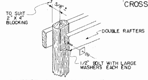
RAFTER CONNECTION DETAIL FOR PERMANENT SHADE
