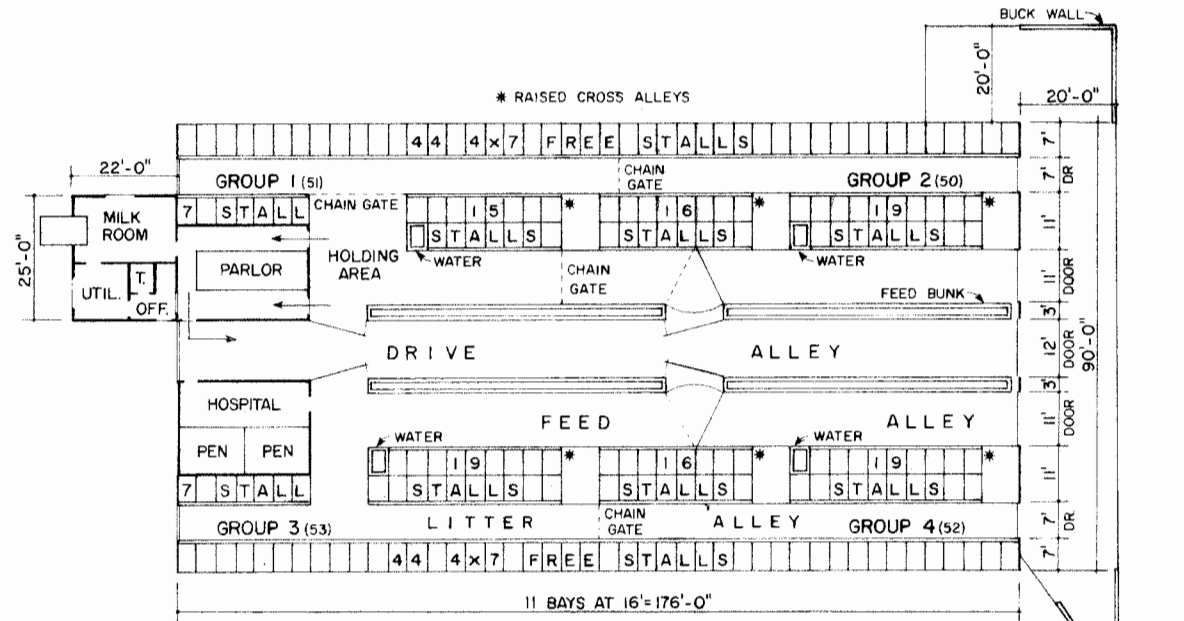
SYSTEM 1: 4 GROUPS PARLOR IN MAIN BARN NO SEPARATE HOLDING AREA 206 STALLS
