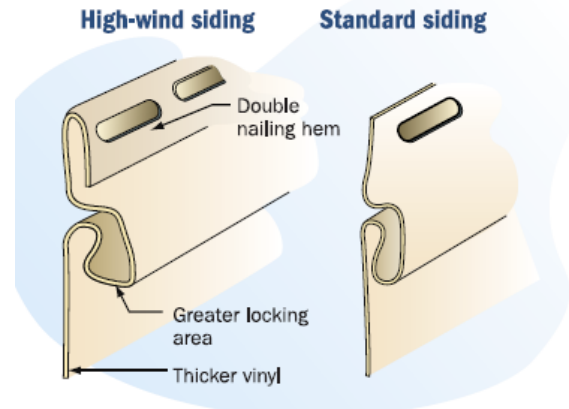
Features of typical high-wind siding and standard siding.
