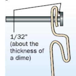
Allow 1/32-inch clearance between the fastener head and the siding panel.
