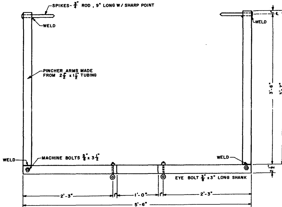
TOP VIEW SCALE 1 1/2" = 1'-0"
