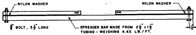
REAR VIEW SCALE 1 1/2" = 1'-0"
