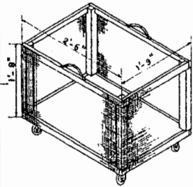
DETAILS OF ROLLING STORAGE BIN
