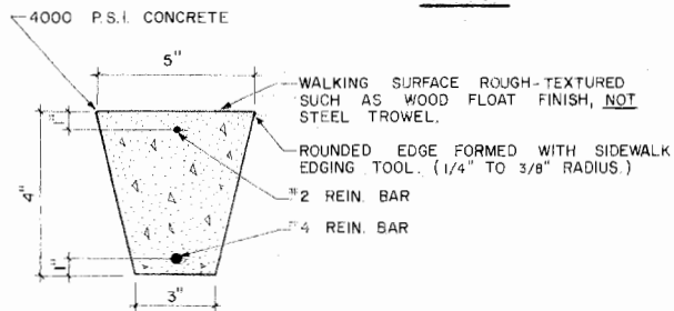
SLAT DETAIL TYPICAL SECTION NOT TO SCALE
