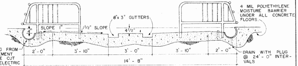
ALTERNATE SECTION "A - A" WITH SHALLOW GUTTER
