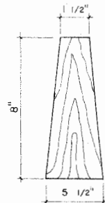
1/2" PLYWOOD SPACER NOT TO SCALE
