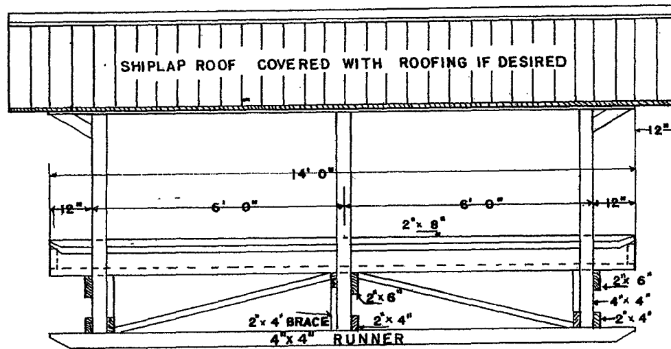
SIDE ELEVATION
