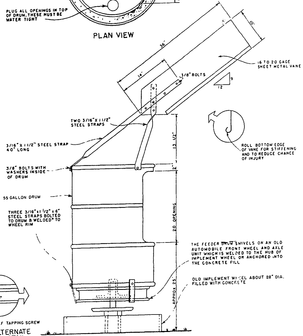
SIDE ELEVATION
