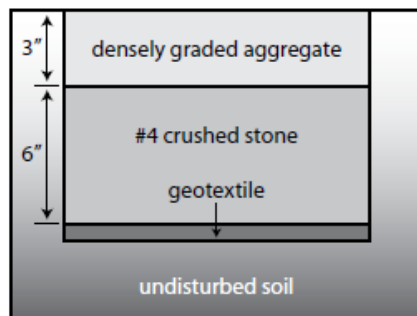
Figure 1. Construction details.
