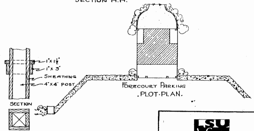
DETAIL OF COLUMN
